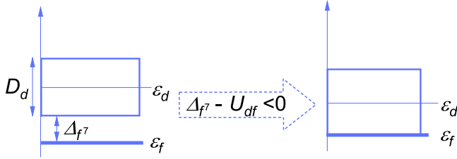
FIG. 4. Schematic of the promotional model in which valence transition is associated with the onsite charge transfer between 4f and 5d states, where U_{df} is the interorbital Coulomb repulsion between the carrier and localized hole on the same site, D_d is the bandwidth of 5d band. Once the gap approaches U_{df} , the valence transition occurs.
