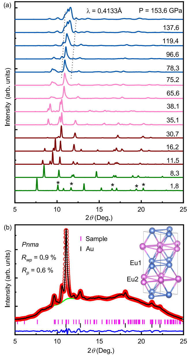
FIG. 3. (a) Selected synchrotron XRD pattern with the subtracted background of Eu at various pressures. (b) Rietveld refinement of the XRD patterns collected at 96.6 GPa for the Pnma structure at room temperature. The red circles, the solid black line, and the green line represent the experimental data, fitted data, and background, respectively. The inset schematic figure shows the local coordination in Eu.
